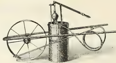
WHEELBARROW SPRAYER
